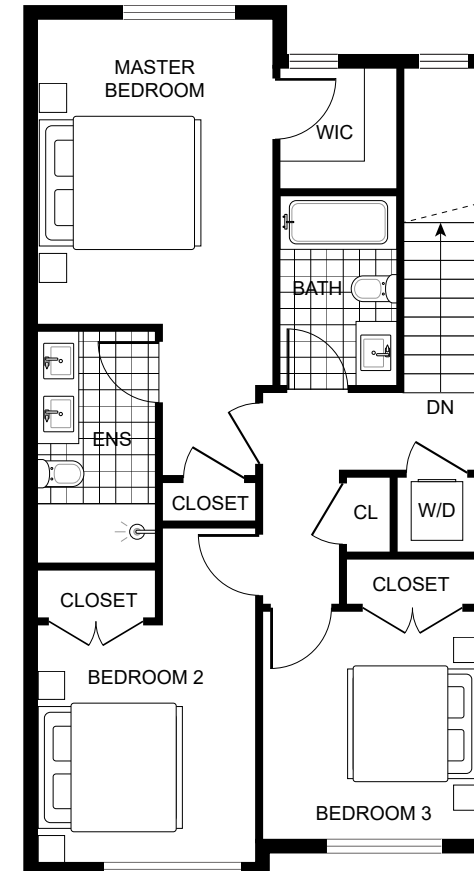
THIRD FLOOR
