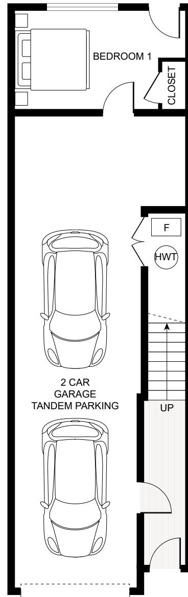
MAIN FLOOR
